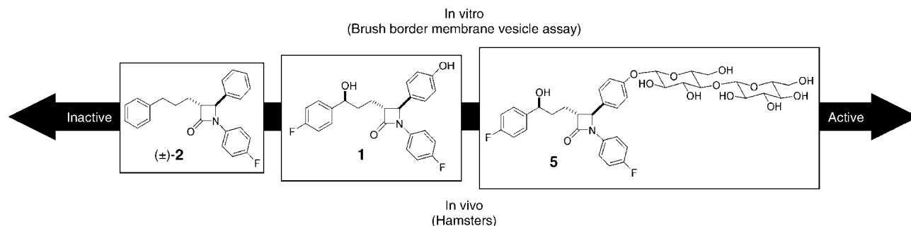
Scheme 1. Correlation between in vitro and in vivo activities with various
