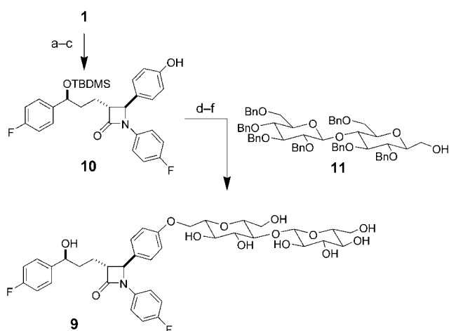
Scheme 3. a) 1 , [16] Ac 2 O, NaOH, i PrOH, 97%; b) TBDMSCl, imid, DMF, 91%; c) Al 2 O 3 (neutral), 70°C, 83%; d) 11 , [24] 1,1'-(azodicarbonyl)dipiperidine, Bu 3 P, THF; e) H 2 , Pd(OH) 2 /C, EtOAc/EtOH, 21% over two steps; f) HF-pyridine, pyridine, THF, 62%. Bn = benzyl, DMF = N,N -dimethylformamide, imid = imidazole, TBDMS = tert -butyl-dimethylsilyl, THF = tetrahydrofuran.
