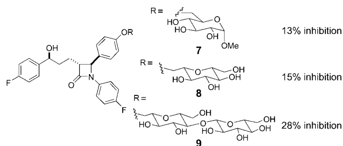
Scheme 2. Nonhydrolyzable glycosides evaluated in the brush border membrane vesicle assay.
