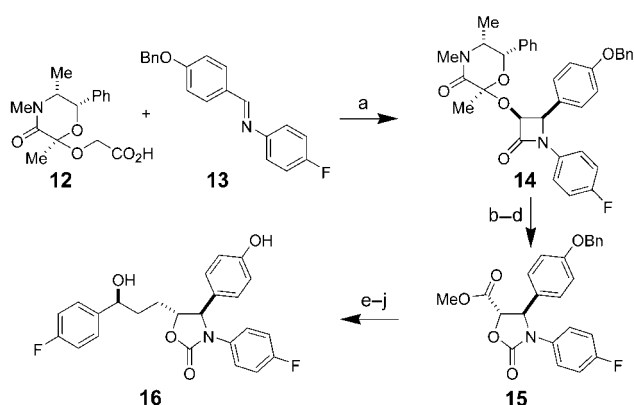
Scheme 4. a) 12 , [26] 13 , [27] (Cl 3 CO) 2 CO, Et 3 N, 0°C→RT, 75%, d.r. = 3:2; b) THF/H 2 O, reflux, 50%; c) NaOMe, MeOH; d) (Cl 3 CO) 2 CO, i Pr 2 NEt, DMAP, CH 2 Cl 2 , -78°C→23°C, 73% over two steps; e) NaBH 4 , EtOH; f) (COCl) 2 , DMSO, Et 3 N, CH 2 Cl 2 , -78°C; g) pFC 6 H 4 COCH=PPh 3 , CH 2 Cl 2 , -78°C→23°C, 82% over three steps; h) H 2 , Pd/C, EtOH; i) ( R )-CBS, [28] BH 3 ·Me 2 S, CH 2 Cl 2 , -20→0°C; j) H 2 , Pd/C, EtOH, 57% over three steps. ( R )-CBS = R -tetrahydro-1-methyl-3,3-diphenyl-1 H ,3 H -pyrrolo(1,2- C )(1,3,2)oxazaborolidine, DMAP = 4-dimethylaminopyridine, DMSO = dimethylsulfoxide.
